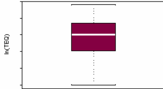
Summary Statistics
