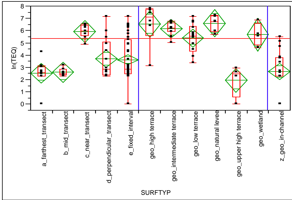
Figure 2: Comparison of means from GeoMorph ® and fixed interval transects from Reach L.
